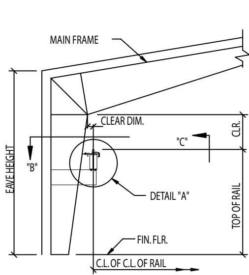
CRANE BEAM AND BRACKET
